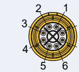
Mating face of Socket
