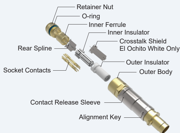
Type II Pin Contact
