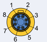
Mating face of Pin
