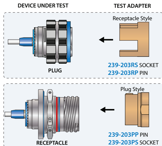
Receptacle Contact Adapter
