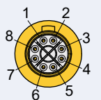
Mating face of Pin
