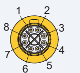
Mating face of Pin
