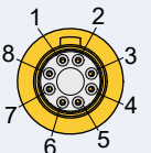
Mating face of Pin
