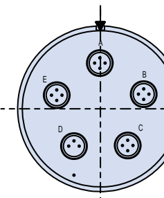
ARRANGEMENT 23Q-05 (IAW PREN 3645-001) 5X SIZE 8 QUADRA
