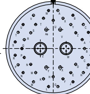
ARRANGEMENT 25Q-46 40X SIZE 20 4X SIZE 16
