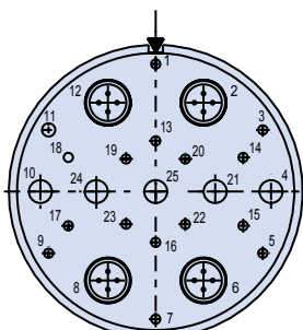
ARRANGEMENT 25Q-26 (IAW PREN 3645-001) 16X SIZE 20, 5X SIZE 12 4X SIZE 8 QUADRA
