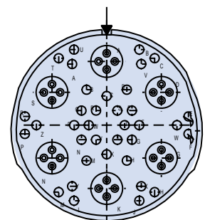
ARRANGEMENT 25Q-17 36X SIZE 22 6X SIZE 8 QUADRA
