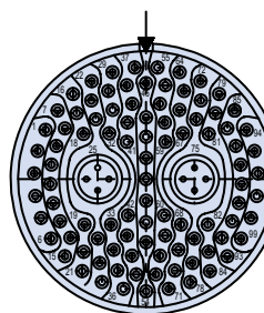
ARRANGEMENT 25Q-07 97X SIZE 22 2X SIZE 8 QUADRA
