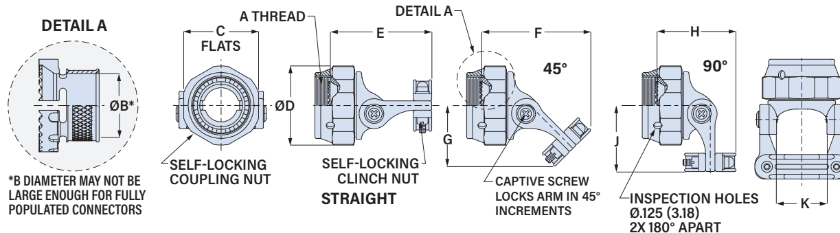
*B DIAMETER MAY NOT BE LARGE ENOUGH FOR FULLY POPULATED CONNECTORS
