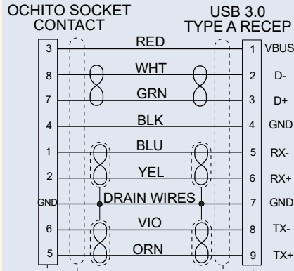
Wiring Diagram 8572-0003-02/06/10 El Ochito ® Socket to USB 3.0 A Recep
