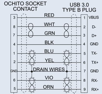
Wiring Diagram 8572-0003-03/07/11 El Ochito ® Socket to USB 3.0 B Plug
