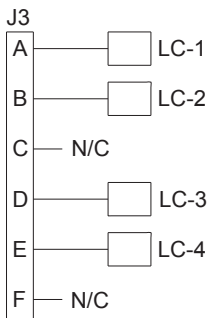
Connection Diagram
