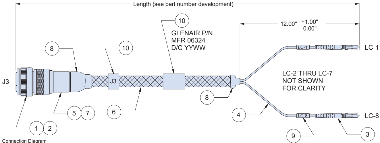
Connection Diagram
