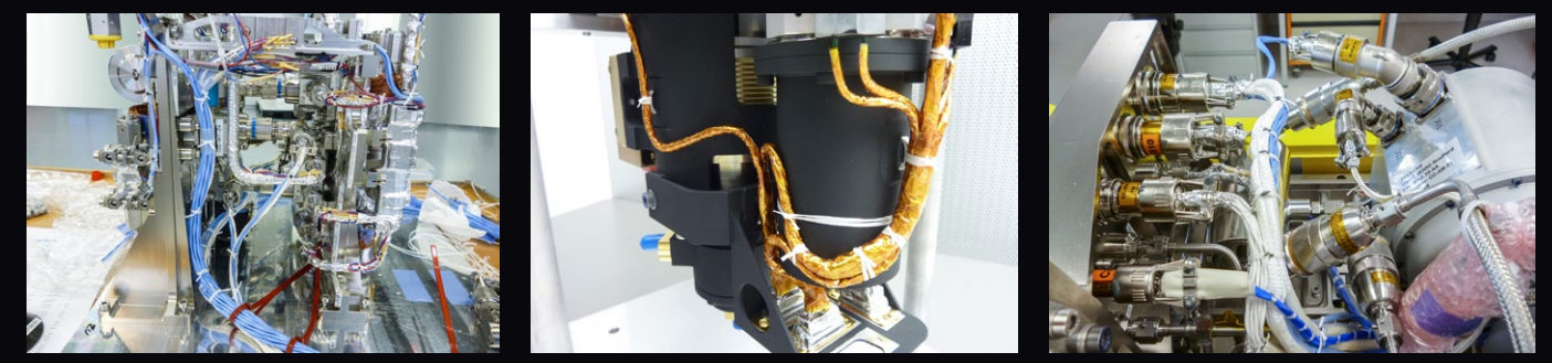
Complex integration and assembly of flight-grade wire harnesses
