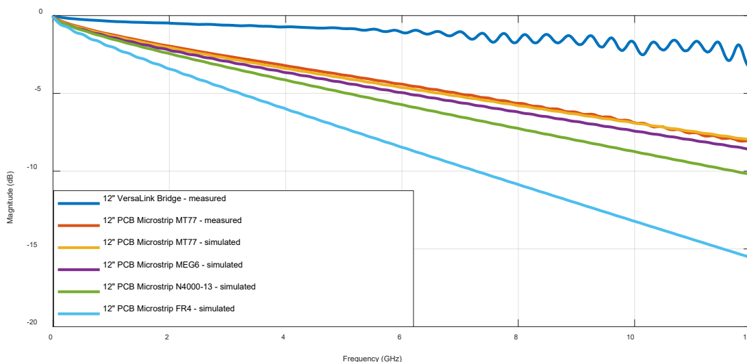
Figure 6 – 12" Link Insertion Losses
