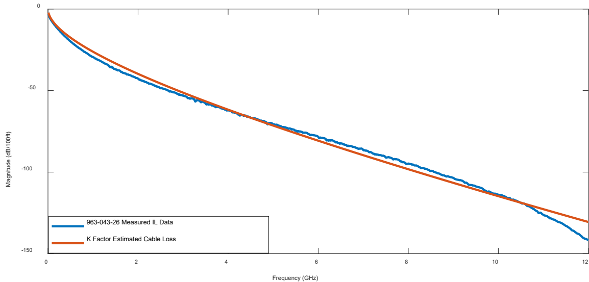
Figure 5 – Measured Cable Loss to Estimate Loss Fit
