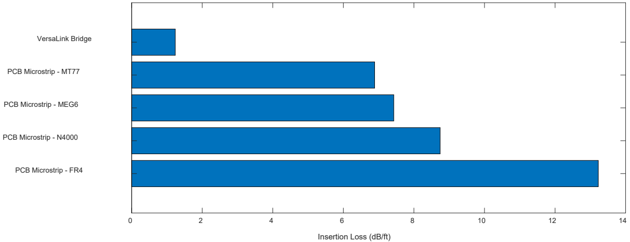
Figure 8 – 12" Link Insertion Loss at 10GHz
