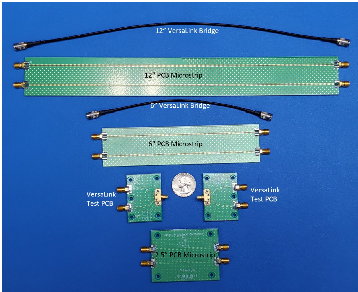
Figure 1 – Comparison Test Articles
