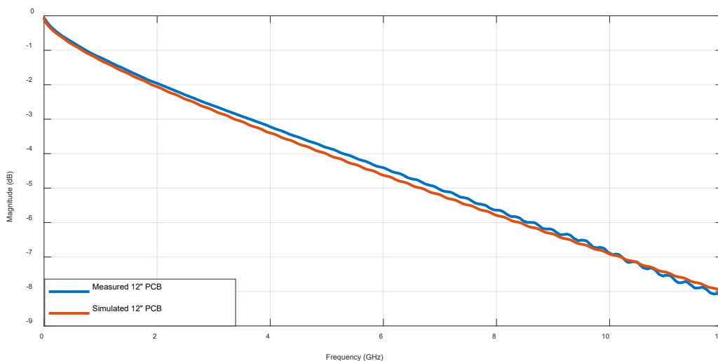
Figure 7 – 12" Link Insertion Losses
