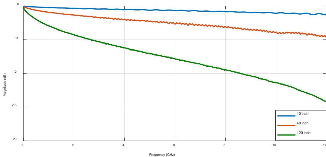
Figure 4 – Twinax Cable Insertion Loss
