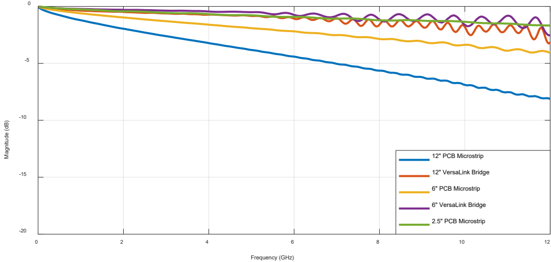
Figure 3 – VersaLink Bridge and PCB Microstrip Insertion Loss
